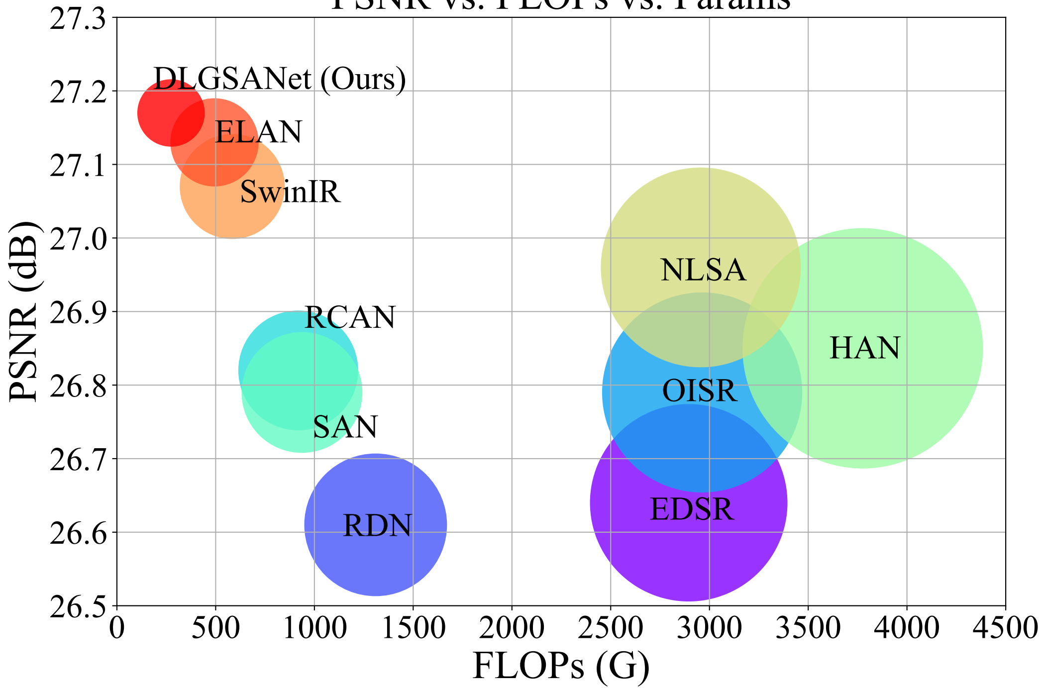
PSNR vs. FLOPs vs. Params
